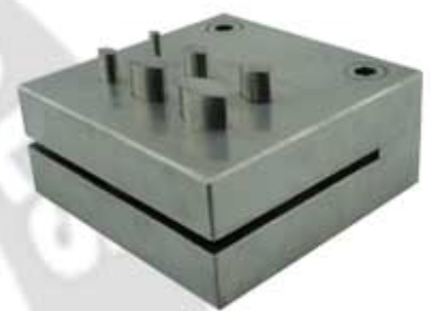
EYE SHAPE DISC CUTTER G.T.W 442.45 SET OF 6 4, 6, 8, 10, 12, 16 MM
